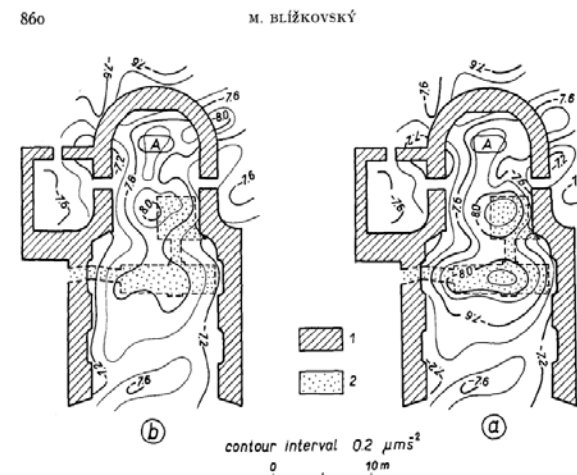
Fig. 10. Maps of Bouguer anomalies in the St. Václav church Tovačov. a) map corrected for gravity effect of walls, b) map corrected for gravity effects of walls and crypts.
