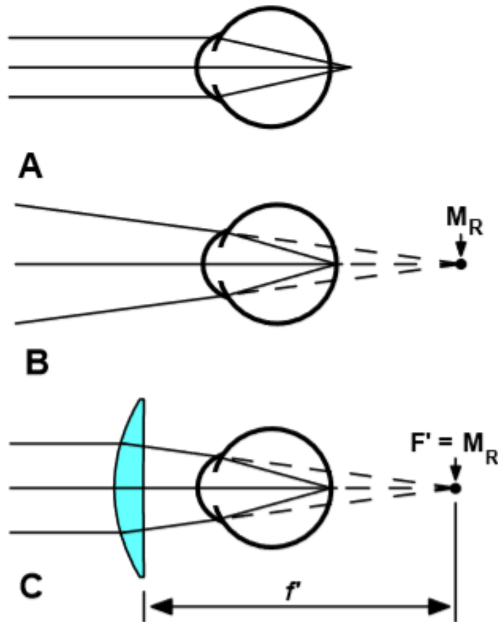
FIGURE 6:13 Plus lens corrections. A) Parallel rays of light from a distant object focus behind the retina of the hyperopic eye. B) Rays of light converging to the far point M_R of the eye focus on the retina. C) The corrective plus lens converges parallel rays from an object at infinity to form a real image at F' , which corresponds to the far point M_R of the eye. This image now becomes a virtual object for the eye that is conjugate with the retina, and forms a clear image upon it.
