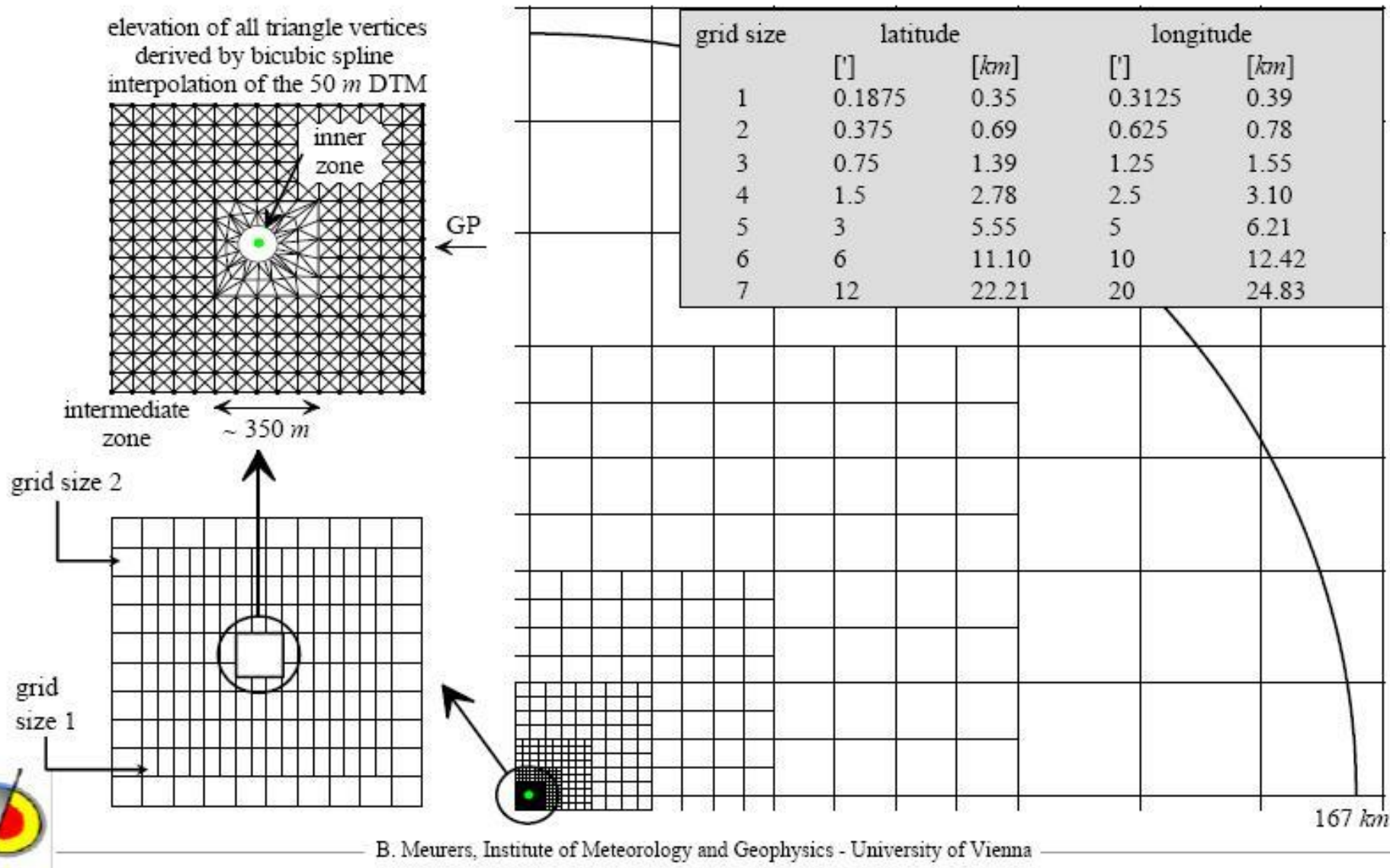
Combination of rectangular prism and polyhedron approximation
