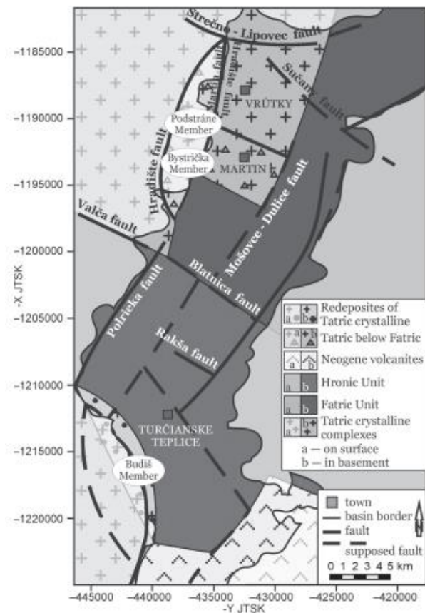
Fig. 10. A sketch of the pre-Tertiary basement structure of the TB.
