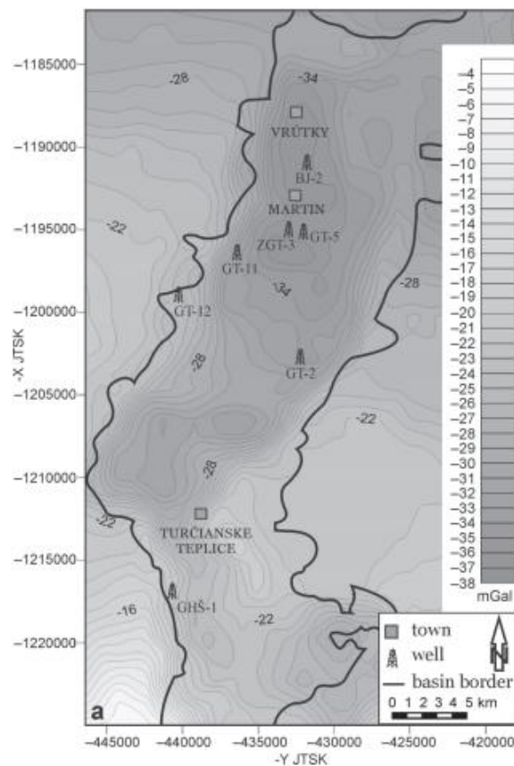
Fig. 7. Stripped gravity map
