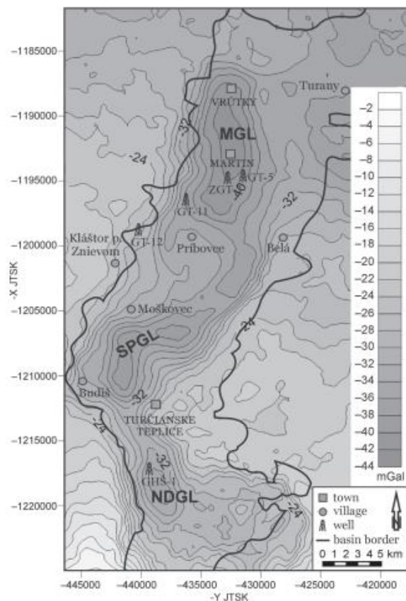
Fig. 3. Complete Bouguer gravity anomaly map calculated by Kučera & Michalík (in Bielík et al. 2007). MGL — Martin gravity low, SPGL — Slovenské Pravno gravity low, NDGL — Nový Dvór gravity low.
