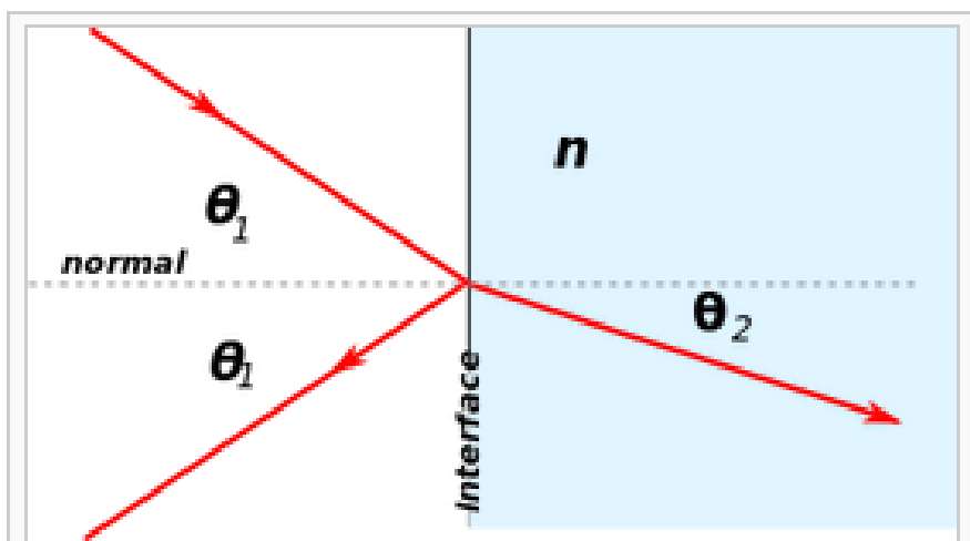
Geometry of reflection and refraction of light rays
