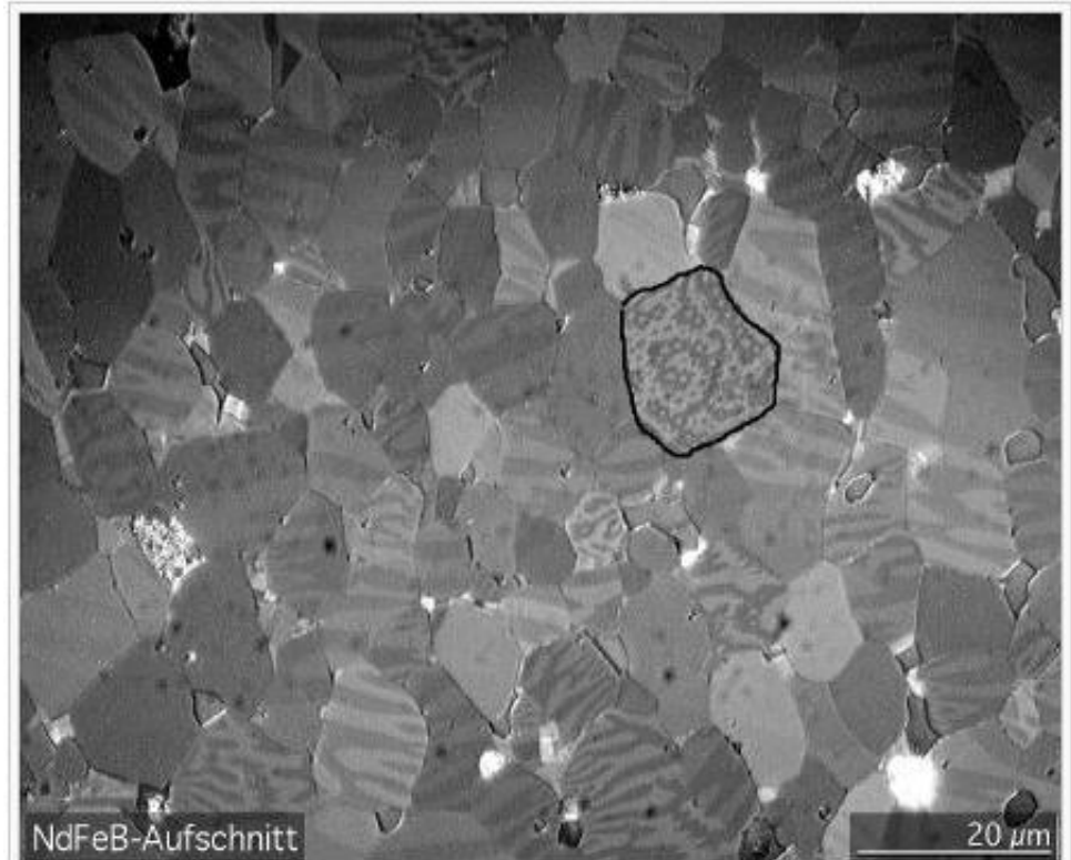
Microcrystalline grains within a piece of NdFeB (the alloy used in neodymium magnets) with magnetic domains made visible with a Kerr microscope. The domains are the light and dark stripes visible within each grain.
