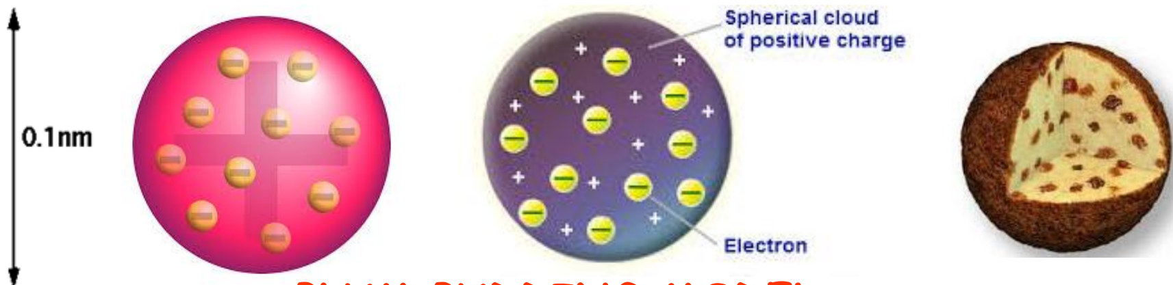
PLUM PUDDING MODEL
