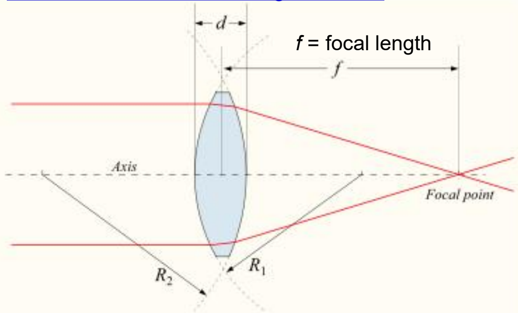
Positive (converging) lens
