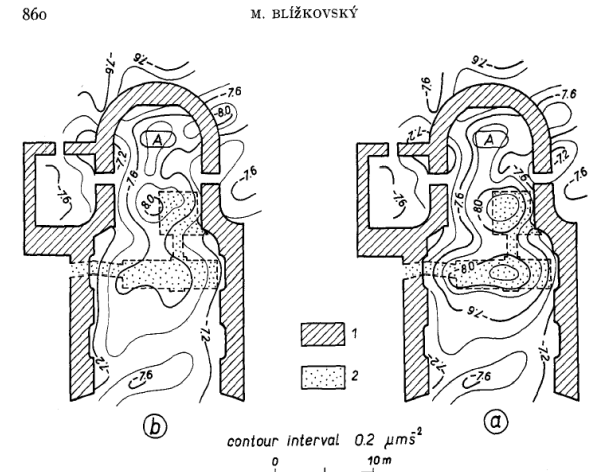
Fig. 10. Maps of Bouguer anomalies in the St. Venceslas church Tovačov. a) map corrected for gravity effect of walls, b) map corrected for gravity effects of walls and crypts.
